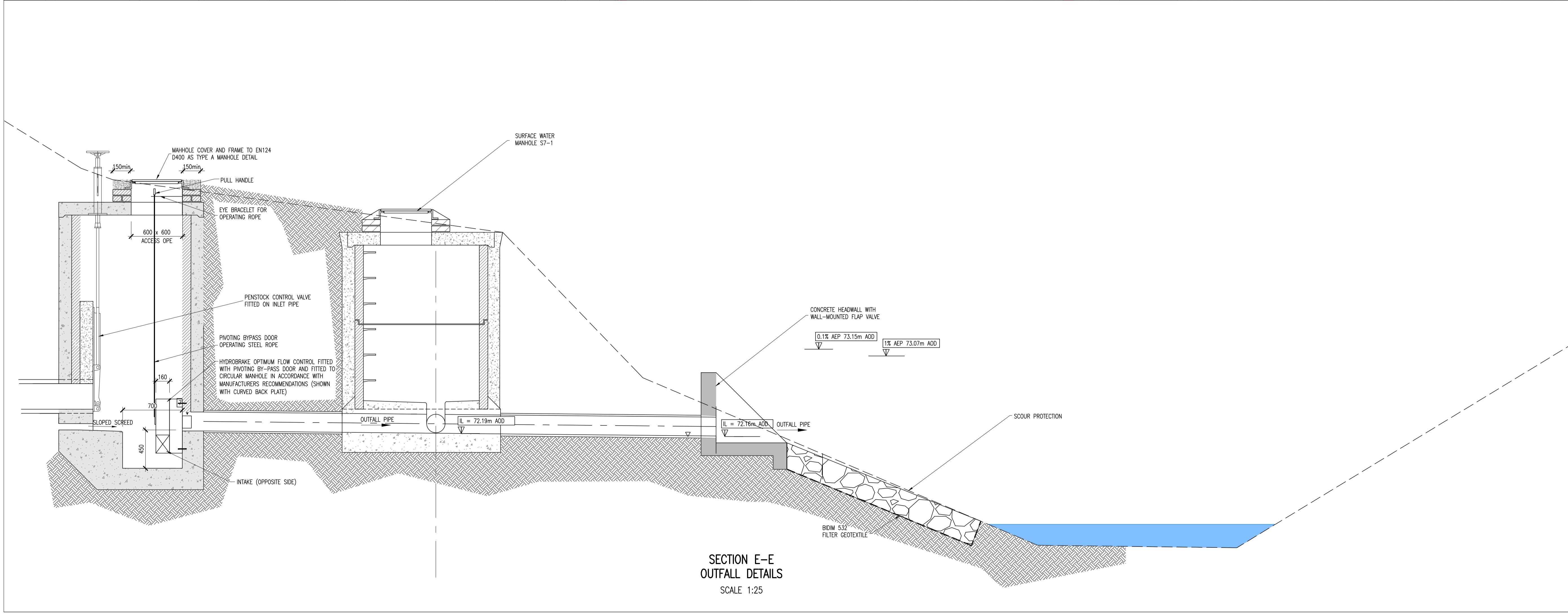
SURFACE WATER OUTFALL SCALE 1:100
